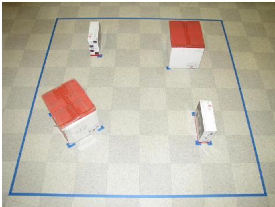
Physical Terrain
